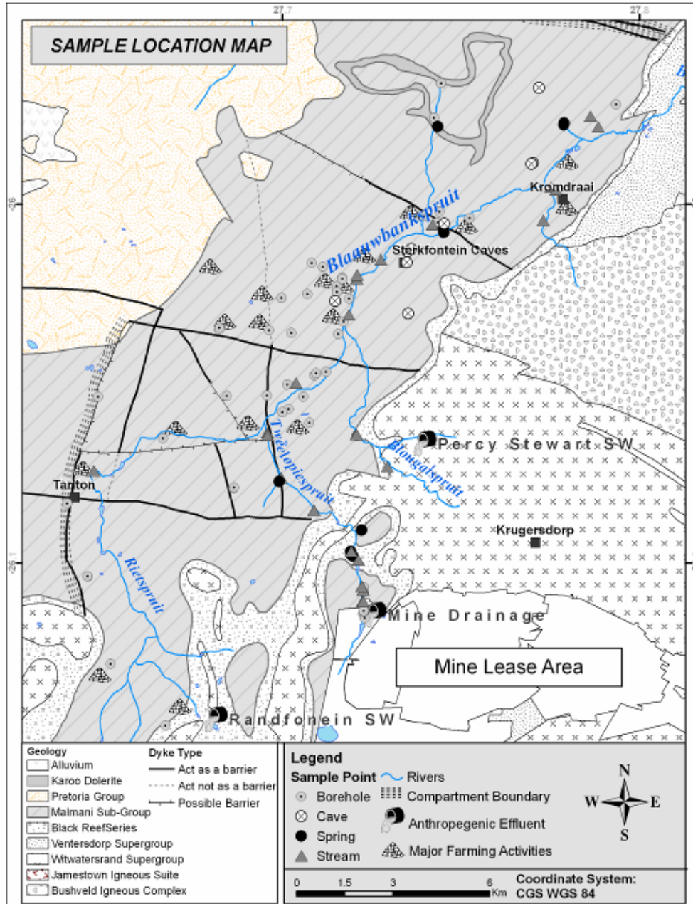
Figure 2. Regional geology and sample locations in the COHWS.
